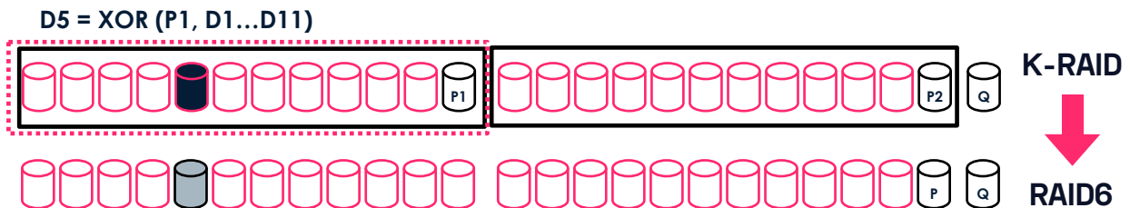
Figure 6: K-RAID flow during SSD failure
