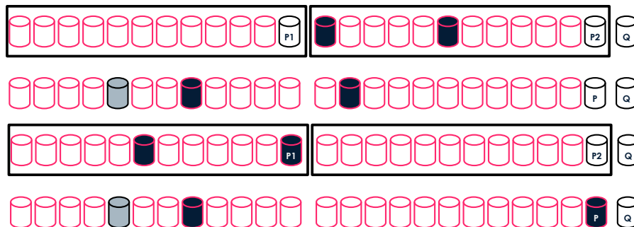
Figure 8: Using the Q Parity for two concurrent SSD failures
